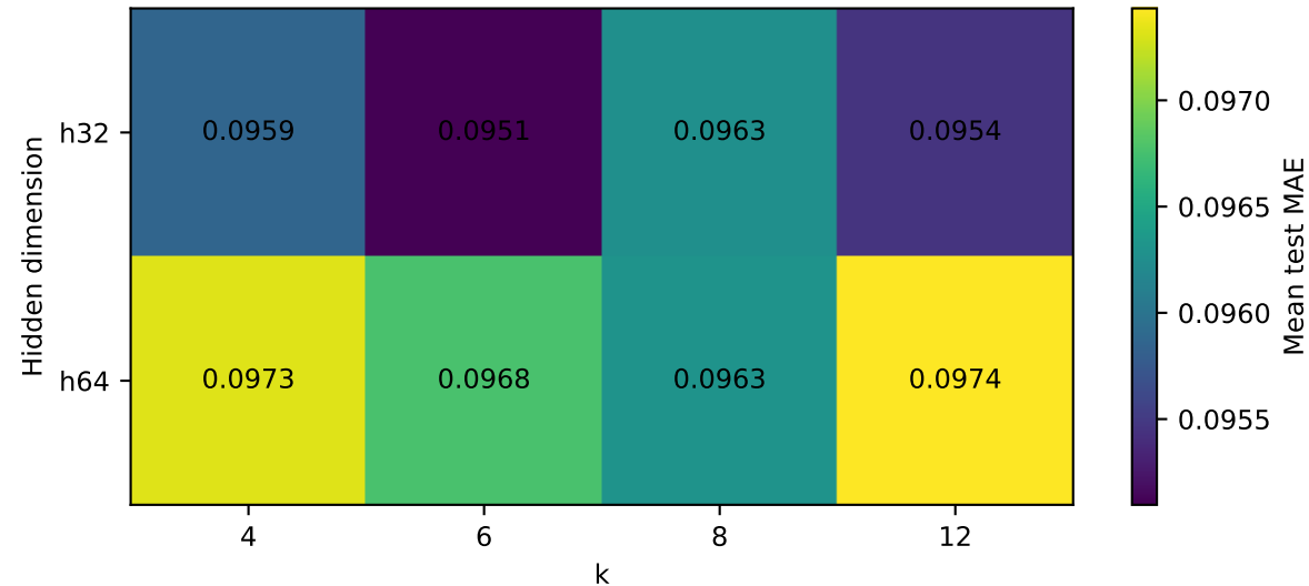
Static GCN: mean test MAE
