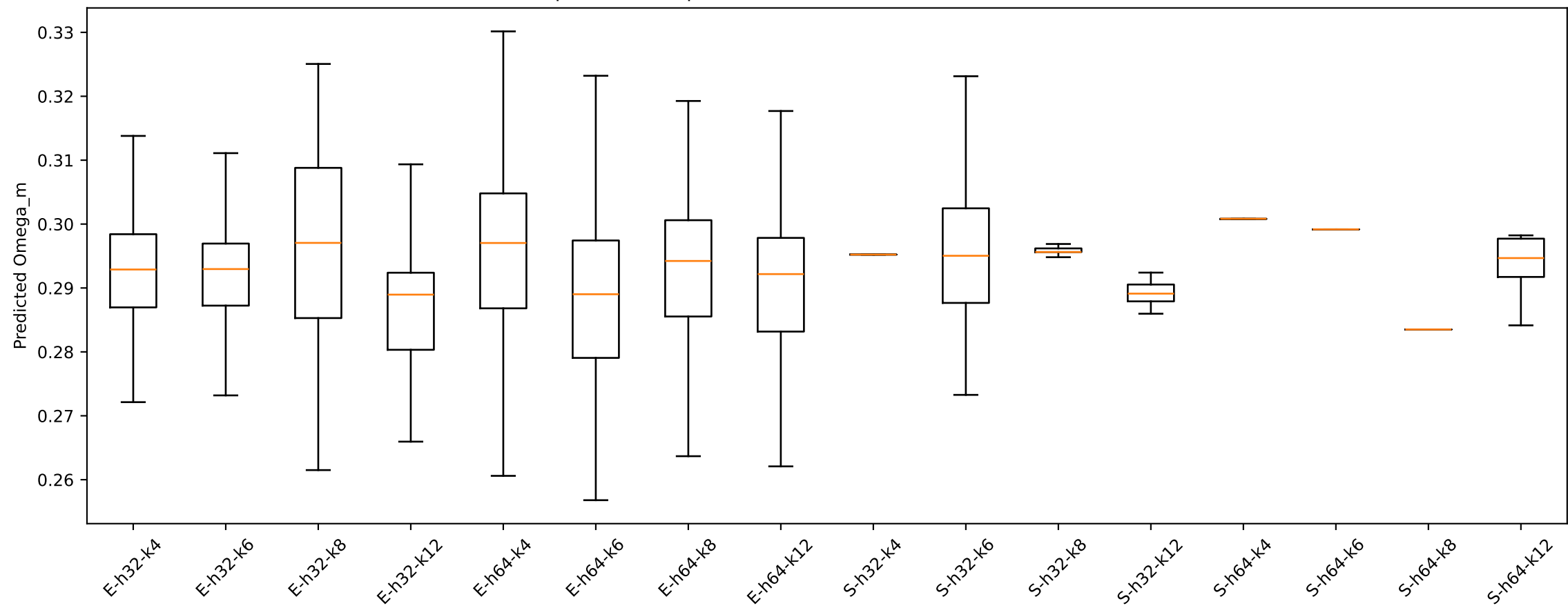
Representative prediction distributions (median-MAE seeds)
