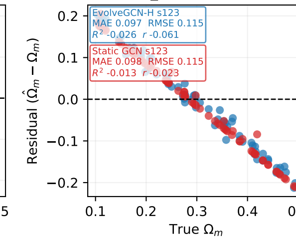
h64_k8 factorial cell
