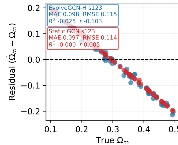
h32_k4 factorial cell
