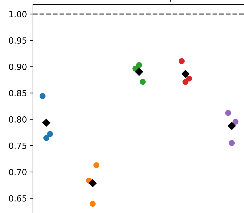
Calibration slope
