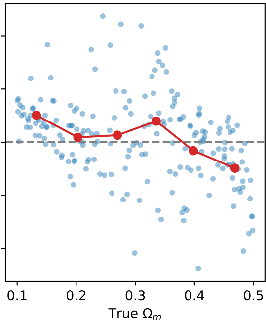
Seed 2025
