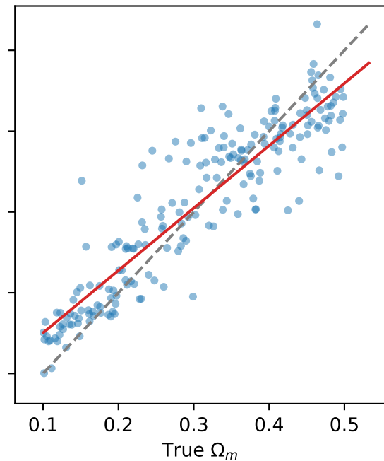
Seed 2025 MAE=0.039, R^2=0.827 , slope=0.77
