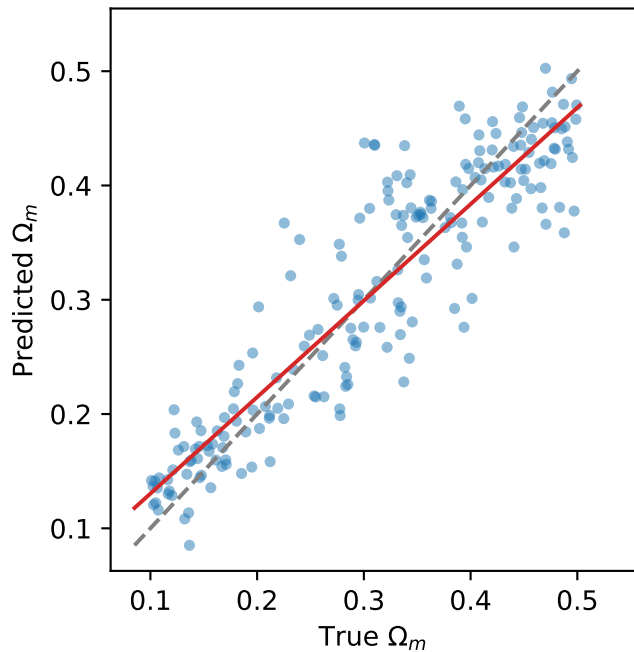
Seed 42 MAE=0.038, R^2=0.837 , slope=0.84
