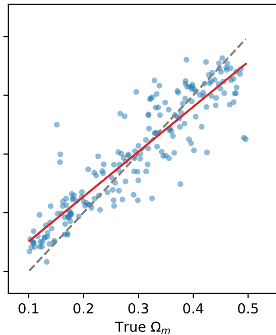
Seed 103 MAE=0.037, R^2=0.815 , slope=0.76
