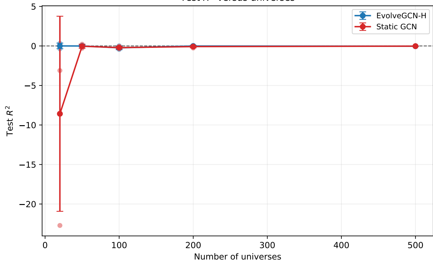
Test R^2 versus universes
