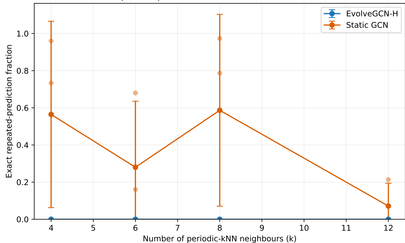
Repeated-prediction behaviour versus k — h64
