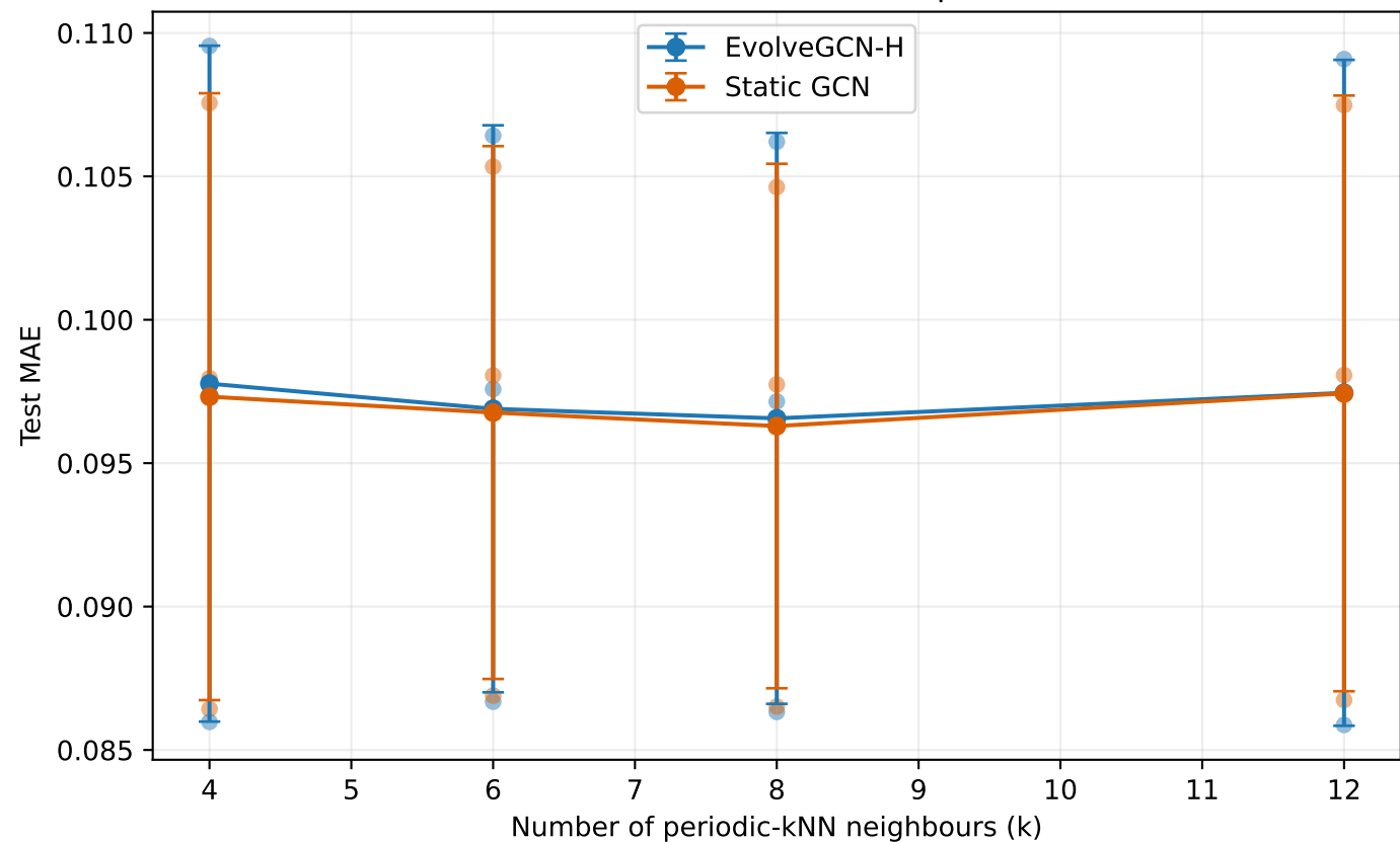
Test MAE versus k — 500U Top100 h64
