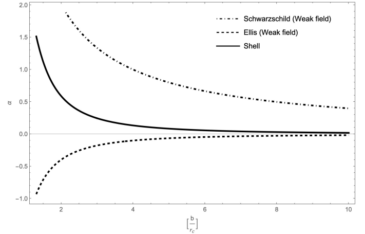
Fig. 6. The shell lensing is weaker than Schwarzschild/Tangherlini(1+3) in the weak field limit.
