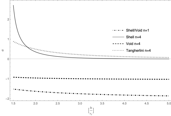
Fig. 7. The coincidence of the shell and void deflection in n = 1 reflects the topological character of (1+1) dimensional gravity, while in n = 4 the shell and Tangherlini geometries exhibit distinct tension- and mass-sourced lensing, respectively.
