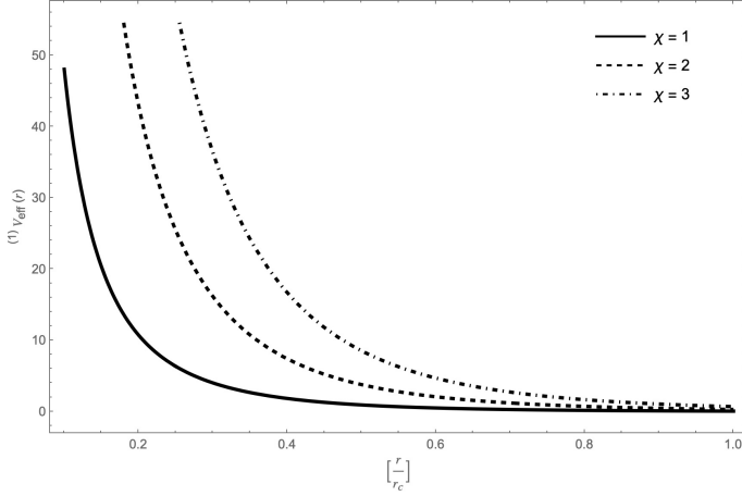
Fig. 3. The Void potential is absolutely impenetrable.
