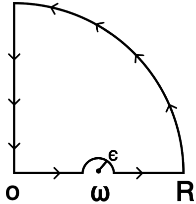
Fig. 1. Contour integration in the first quadrant of the complex plane.
