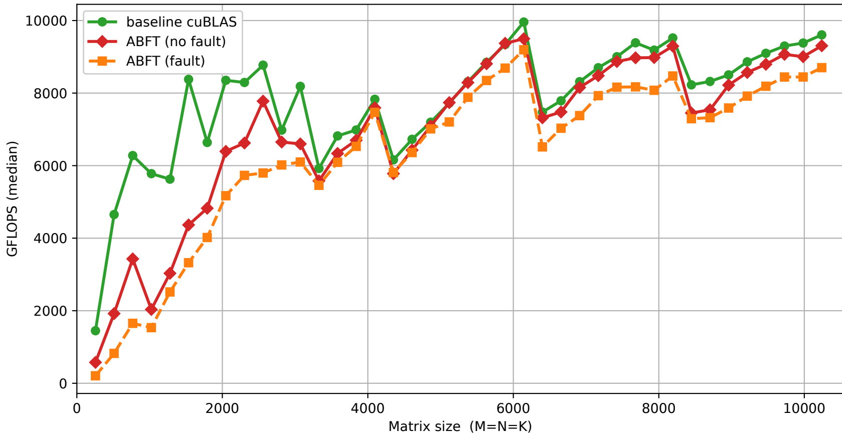
Throughput vs size — baseline vs ABFT ( \pm fault)
