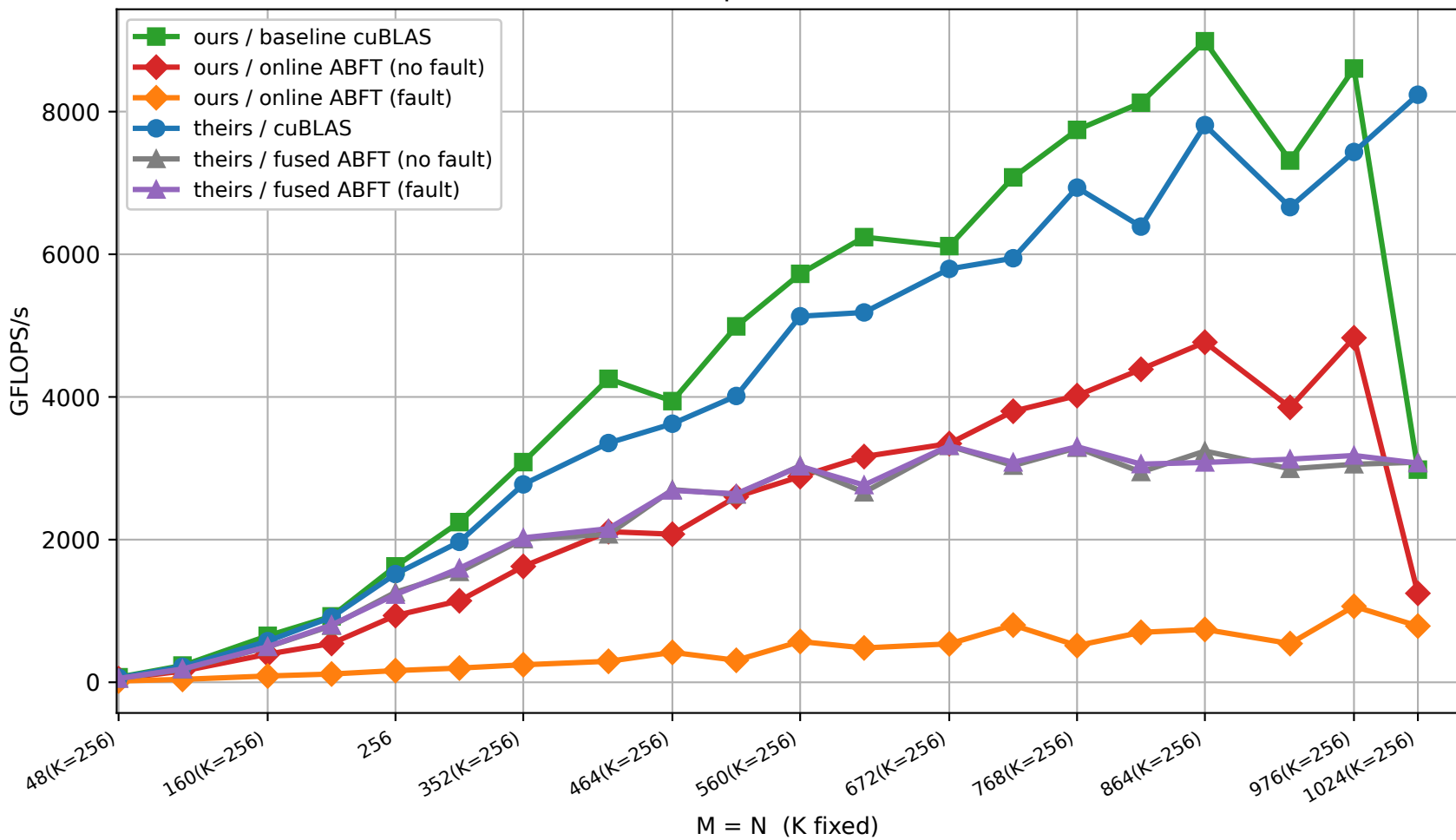
GFLOPS — Non-square, small ( M=N , K=256 )
