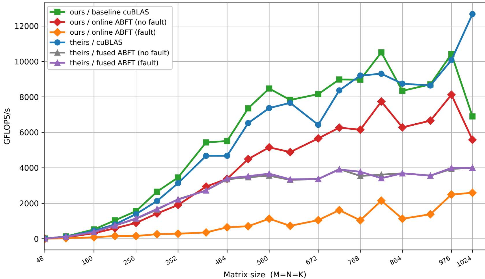
GFLOPS — Square, small ( M=N=K , \sim 50 -1024)
