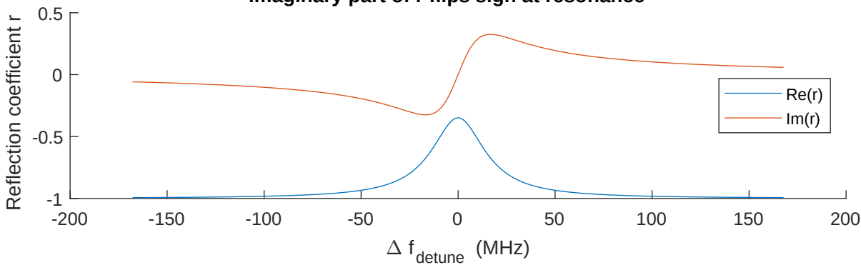
Imaginary part of r flips sign at resonance
