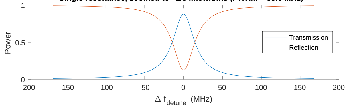
Reflection phase change over shown span: -7^\circ
