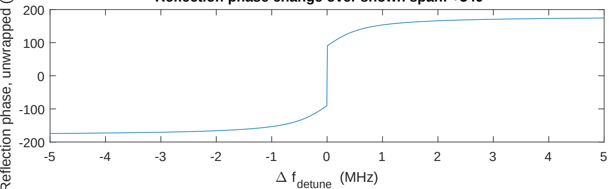
Imaginary part of r flips sign at resonance
