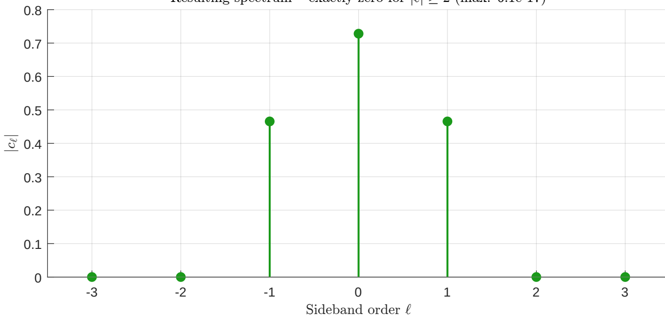
Resulting spectrum – exactly zero for |\ell| \geq 2 (max: 6.1e-17)
