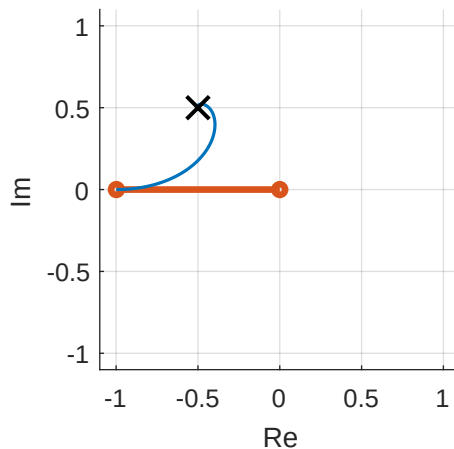
(b) \Delta f_{\text{detune}} = +0.5\Delta\nu_{\text{FWHM}}
