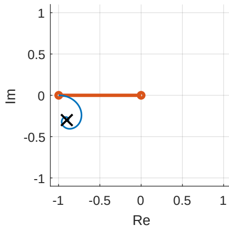
(e) \Delta f_{\text{detune}} = -1.5\Delta\nu_{\text{FWHM}}
