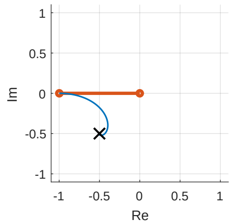
(c) \Delta f_{\text{detune}} = -0.5\Delta\nu_{\text{FWHM}}
