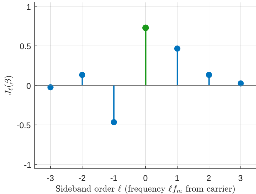
Optimal: \beta = 1.082 , J_0J_1 = 0.339
