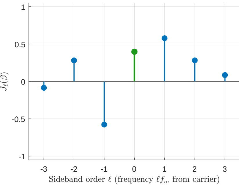
Over-modulated: \beta = 1.700 , J_0J_1 = 0.230
