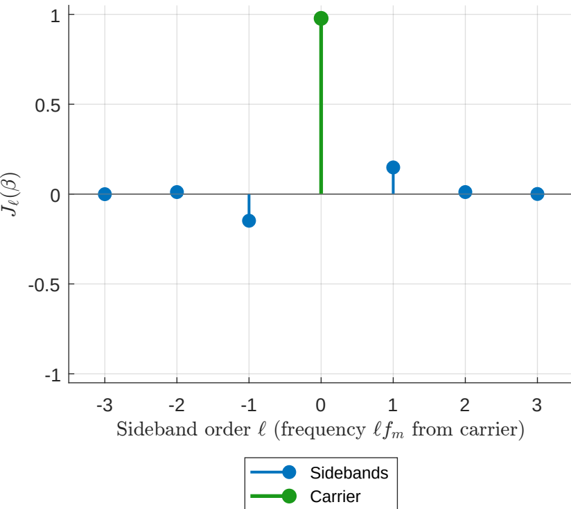
Under-modulated: \beta = 0.300 , J_0J_1 = 0.145
