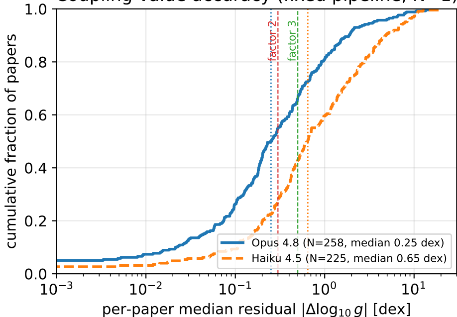
Coupling-value accuracy (fixed pipeline, N=1)
