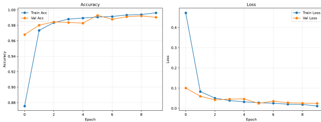
Fig. 1. Kurva training dan validasi MobileNetV3-Small fine-tune (E4).
