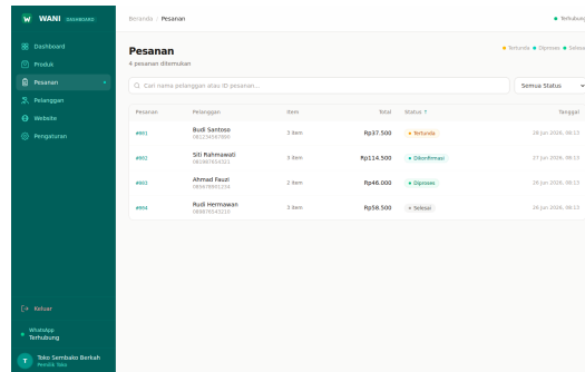
Gambar 8: Halaman Pesanan
