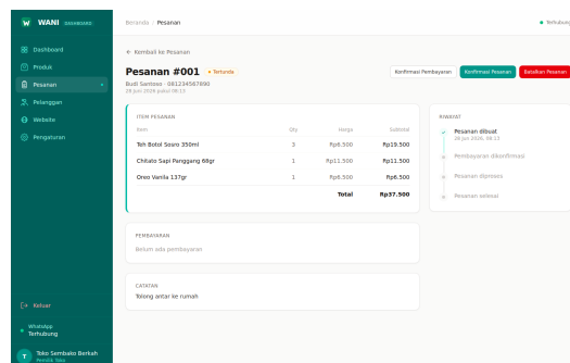
Gambar 9: Detail Pesanan
