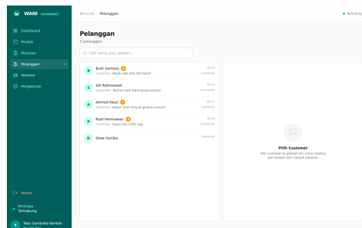
Gambar 10: Halaman Pelanggan
