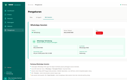
Gambar 14: Pengaturan WhatsApp
