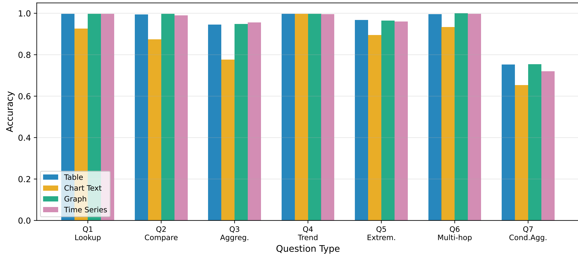
Accuracy by Question Type and Format (Averaged Across 6 Models)
