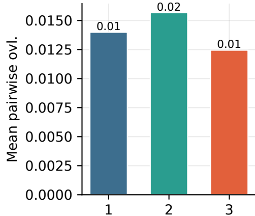
Cascade Overlap ↓
