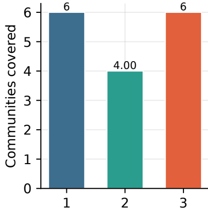
Comm. Cov. ↑
