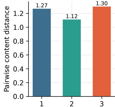
Emb. Dist. ↑
