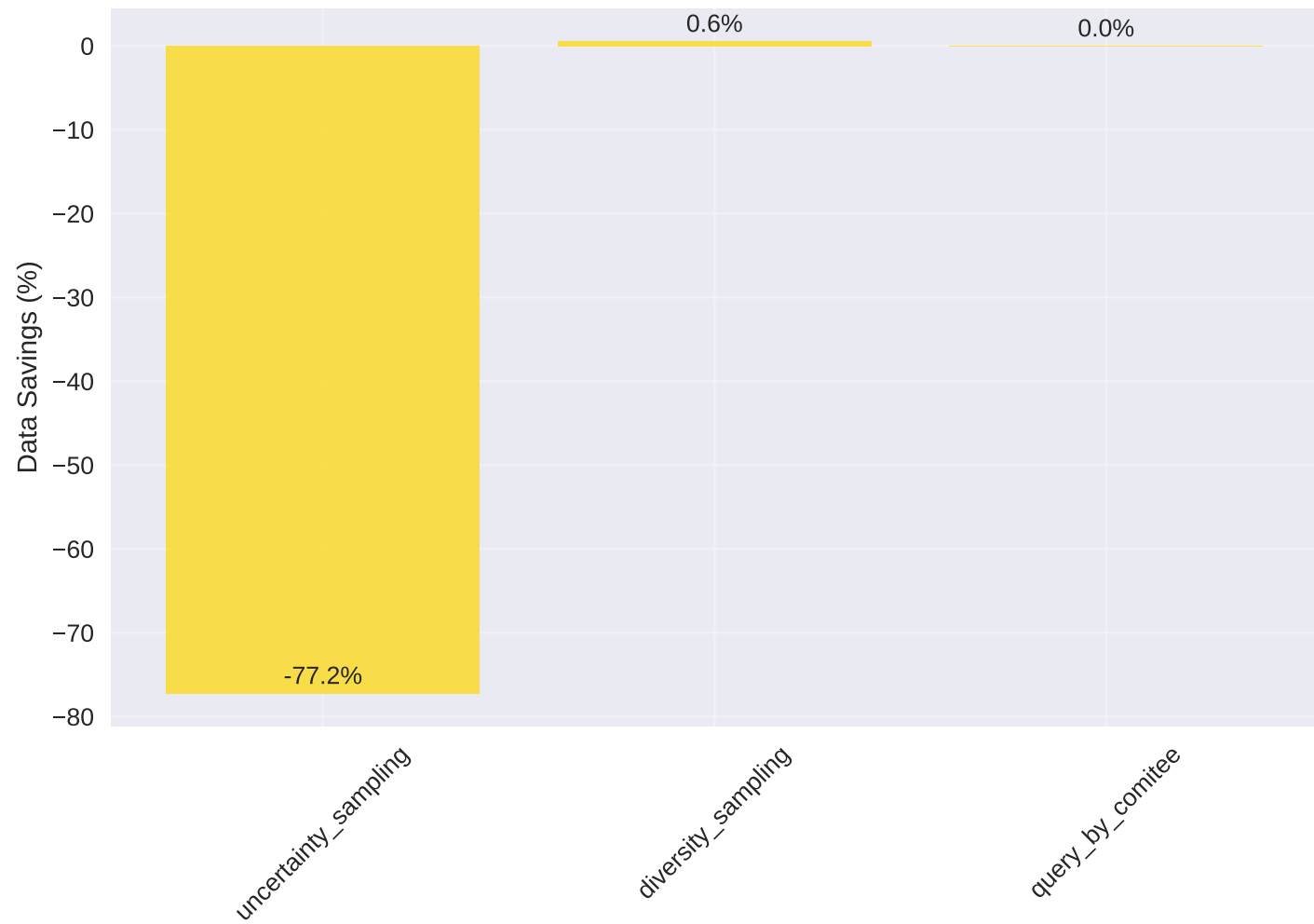
Training Data Savings for Same Macro F1
