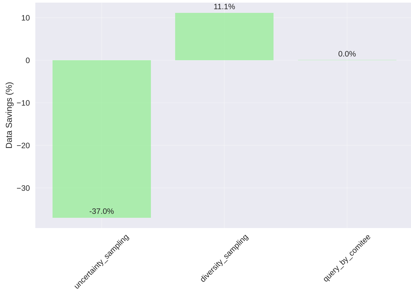
Training Data Savings for Same Accuracy
