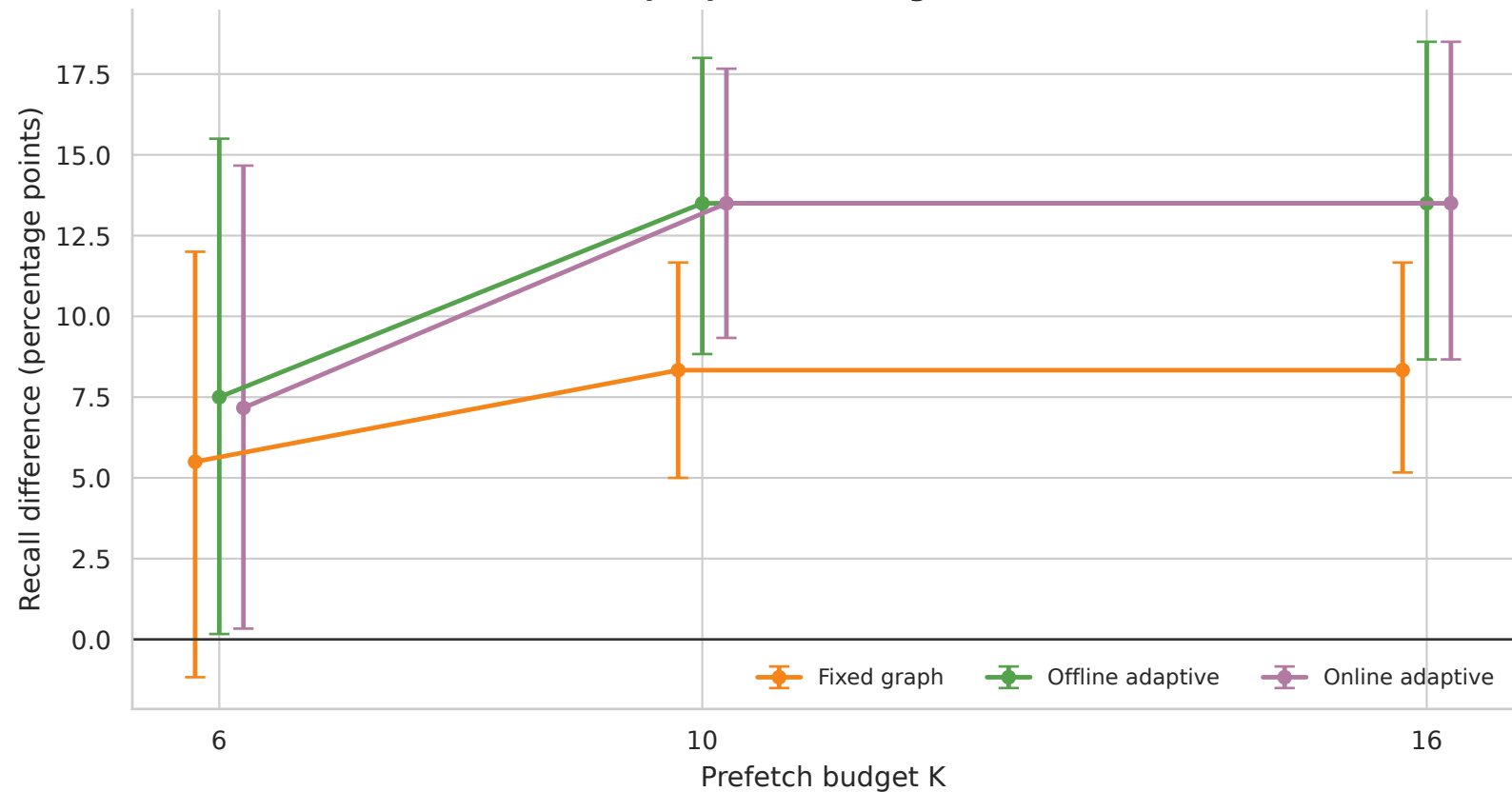
Llama-Hotpot paired recall gain over cosine
