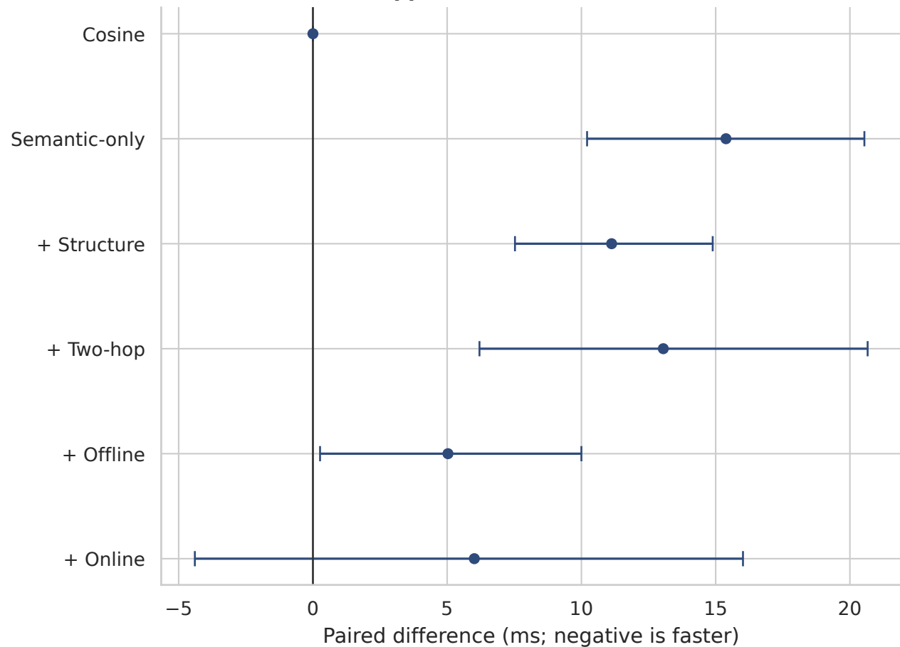
Application TTFT vs cosine
