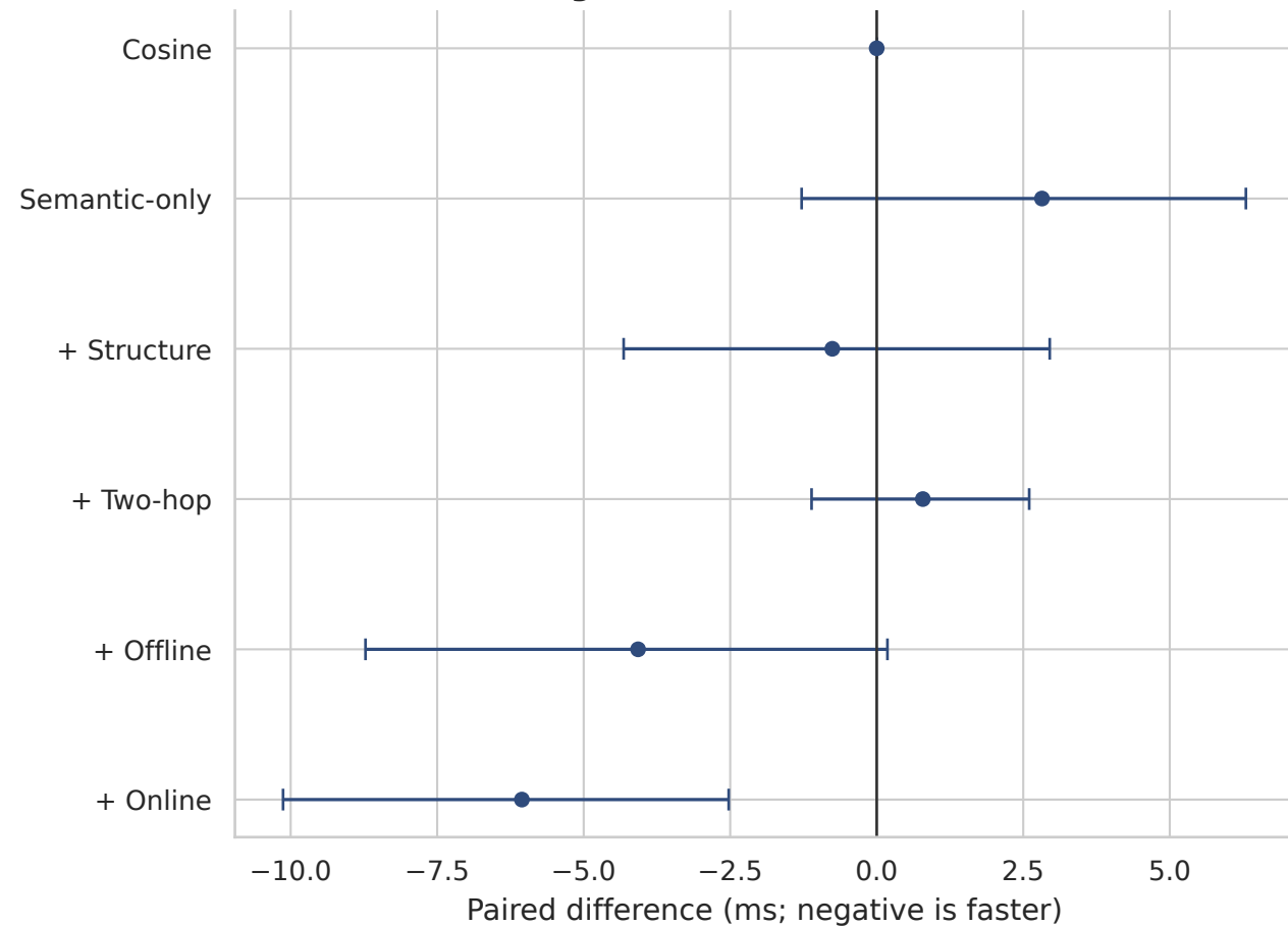
Target-service TTFT vs cosine
