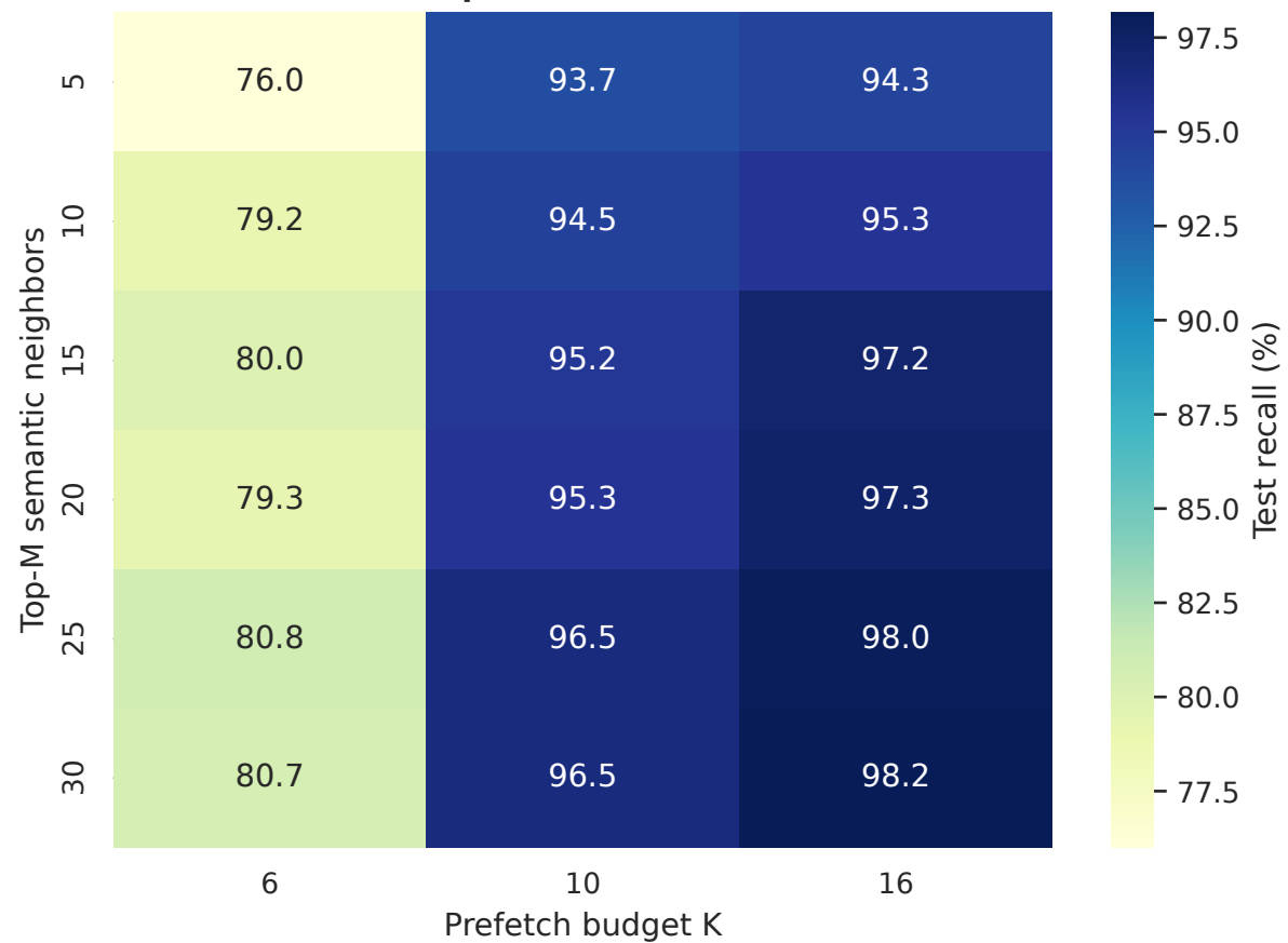
Offline adaptive held-out test recall
