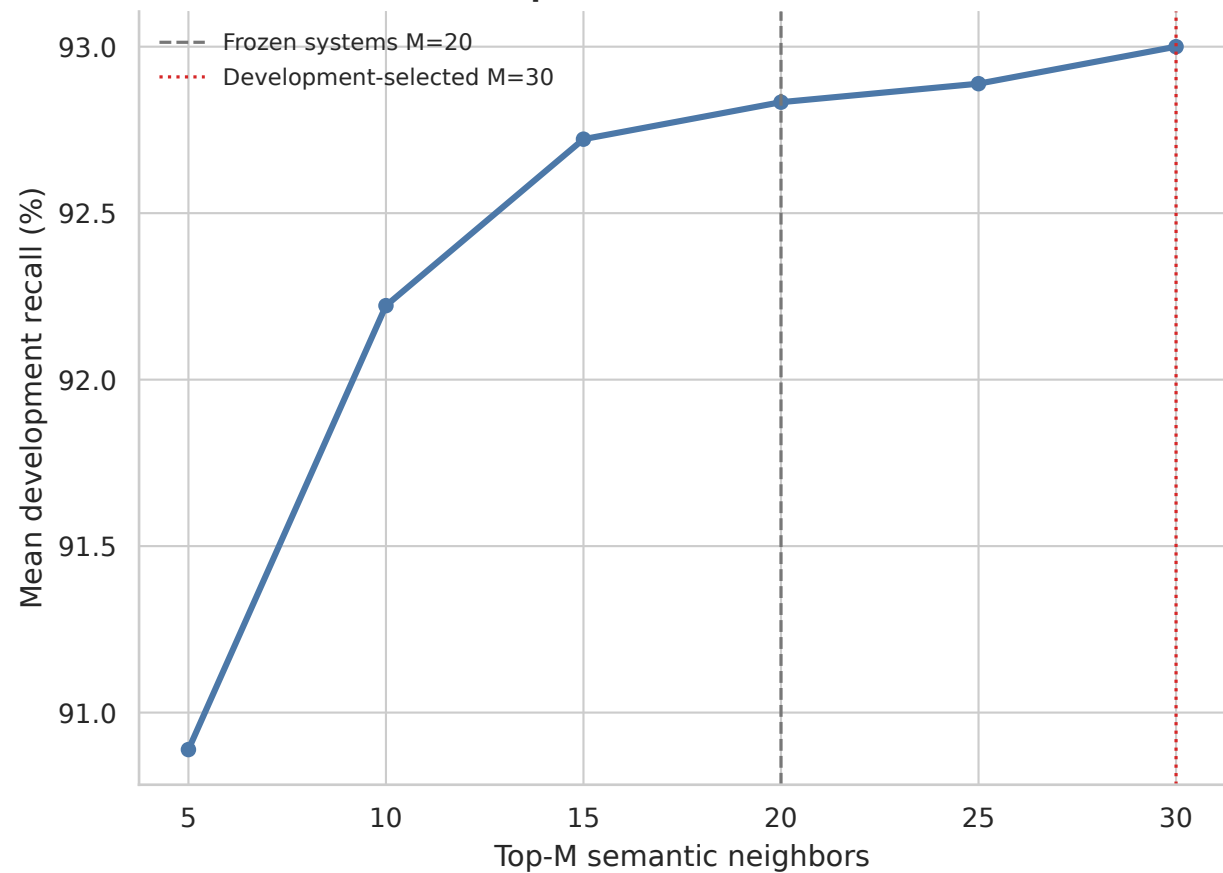
Development selection across M
