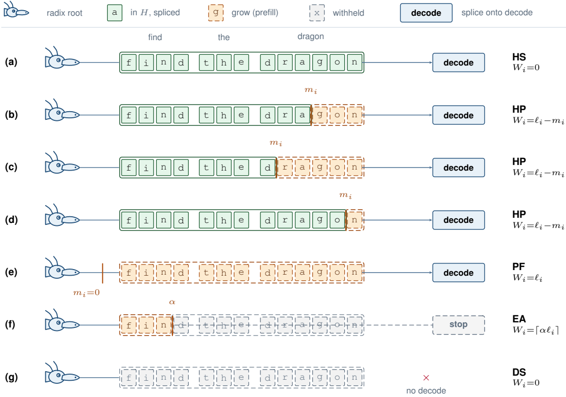
Figure 5. Seven cuts of “find the dragon.” The dragon head is the radix root; the body is one residual. Green tokens are full pages in H and are spliced onto decode. Orange tokens are absent from H and are grown by prefill. Gray tokens are withheld. Chips stand in for tokens: a real hit ends on a full page, and each row is a different value of m_i . (a) The body is a hit ( HS , m_i = \ell_i , W_i = 0 ). (b) The front half “dra” is in the tree and “gon” grows ( HP , W_i = \ell_i - m_i ). (c) The cut falls after “d”. (d) The cut falls before the last character. (e) A miss grows the body from the neck ( PF , m_i = 0 , W_i = \ell_i ); the head stays the alias. (f) The first \lceil \alpha \ell_i \rceil tokens grow and the kernel stops ( EA ). (g) A repeated loop is withheld ( DS , W_i = 0 ). A low score that is not a loop is not this row: it is prefilled, then decoded for a probe (Algorithm 1).
