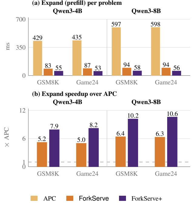
Figure 9. Expand versus APC on the same four runs as Table 9. (a) Expand milliseconds per problem. (b) Speedup of that expand over APC. The dashed line is 1\times . ForkServe is 5.0-6.4\times and ForkServe+ is 7.9-10.6\times . Decode in Table 9 does not repeat that ratio: the step decodes sit in the ForkServe decode column, so ForkServe end-to-end stays with APC.
