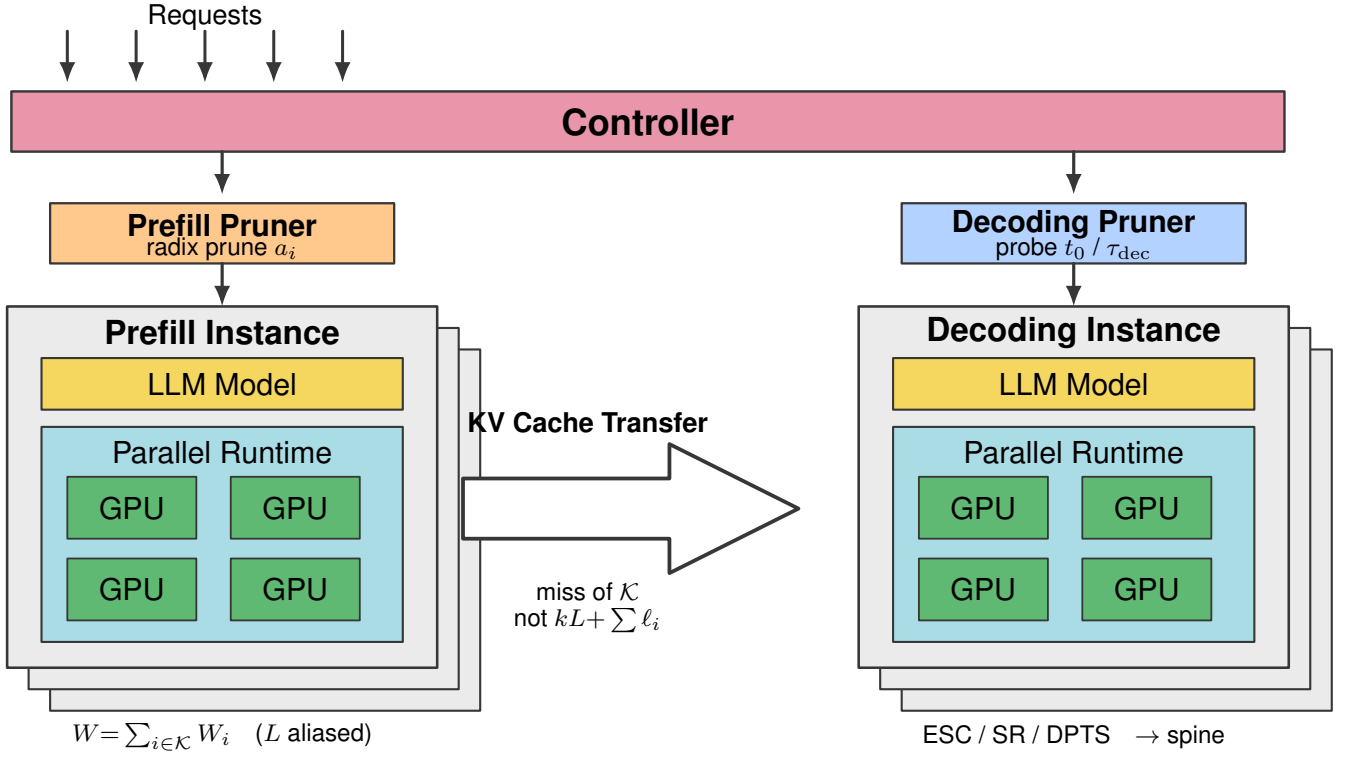
Figure 1: PD-Prune runtime architecture (DistServe-style). Requests hit the controller, then a Prefill Pruner (radix prune a_i ) or a Decoding Pruner (probe t_0 ) before the corresponding instance. Only the miss tail of \mathcal{K} crosses the KV connector; abort retains the spine.
