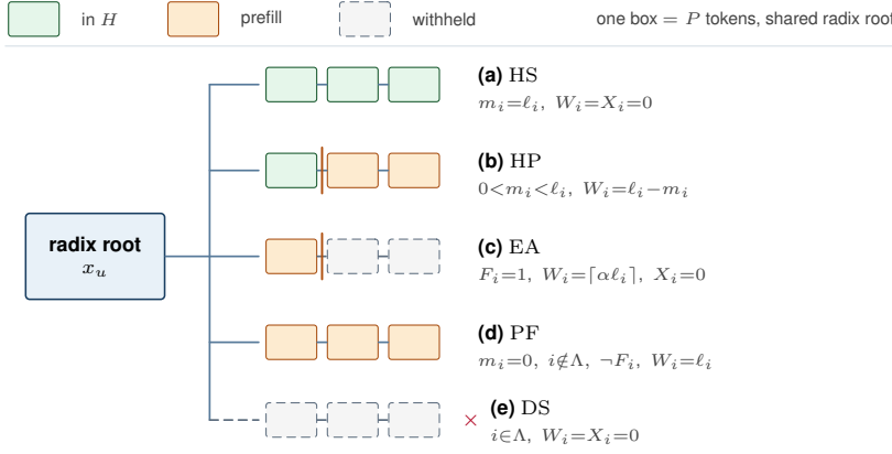
Figure 11: One radix tree, five actions ((4)–(6)). The root is the aliased trunk x_u . Each edge is one page of P tokens. Green pages are in H ; orange pages are prefilled; gray pages are withheld. (a) HS: m_i = \ell_i , W_i = X_i = 0 . (b) HP: 0 < m_i < \ell_i , W_i = \ell_i - m_i . (c) EA: m_i = 0 , F_i = 1 , W_i = \lceil \alpha \ell_i \rceil , X_i = 0 . (d) PF: m_i = 0 , i \notin \Lambda , \neg F_i , W_i = \ell_i . (e) DS: i \in \Lambda , W_i = X_i = 0 . A score below \tau with i \notin \Lambda is prefilled and probed (Algorithm 1).
