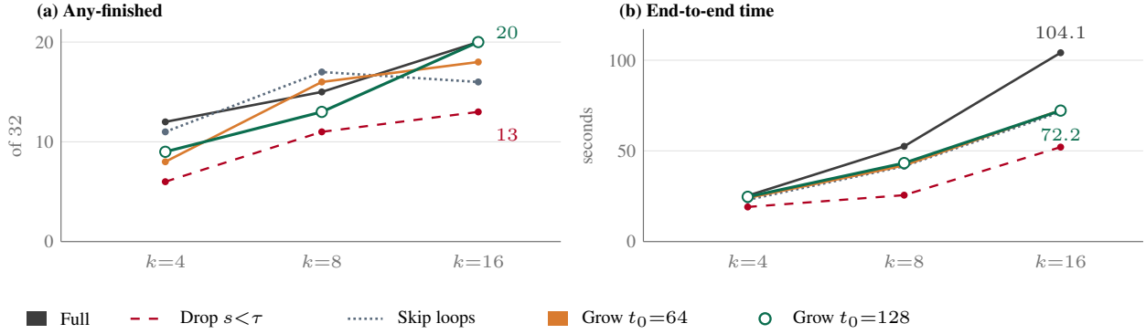
Figure 5. Probe admission on MATH-500 (Table 7). Any-finished counts a problem only when a full-budget branch matches. Dropping every s < \tau is the fast curve and the low count. Grow t_0=128 returns to 20/32 at k=16 and cuts 104.1 s to 72.2 s. At k=8 , grow t_0=64 is 16/32 in 42.0 s, above the full fan-out.
