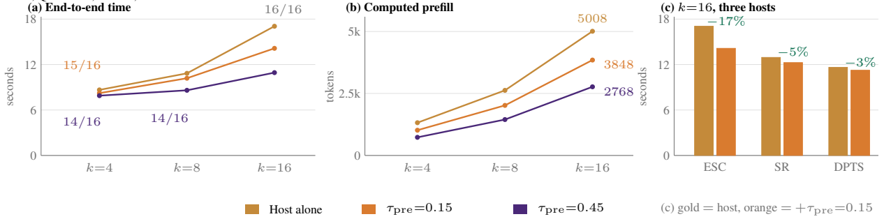
Figure 6. Prefill threshold on GSM8K (Tables 8 and 9). (a) Wall-clock under ESC. Labels are any-finished. \tau_{pre}=0.45 is 14/16 at k=4 and k=8 , and 16/16 at k=16 . (b) Computed prefill tokens, -23\% at 0.15 and -45\% at 0.45. (c) The same 0.15 threshold in front of each host at k=16 . Every row stays 16/16.
