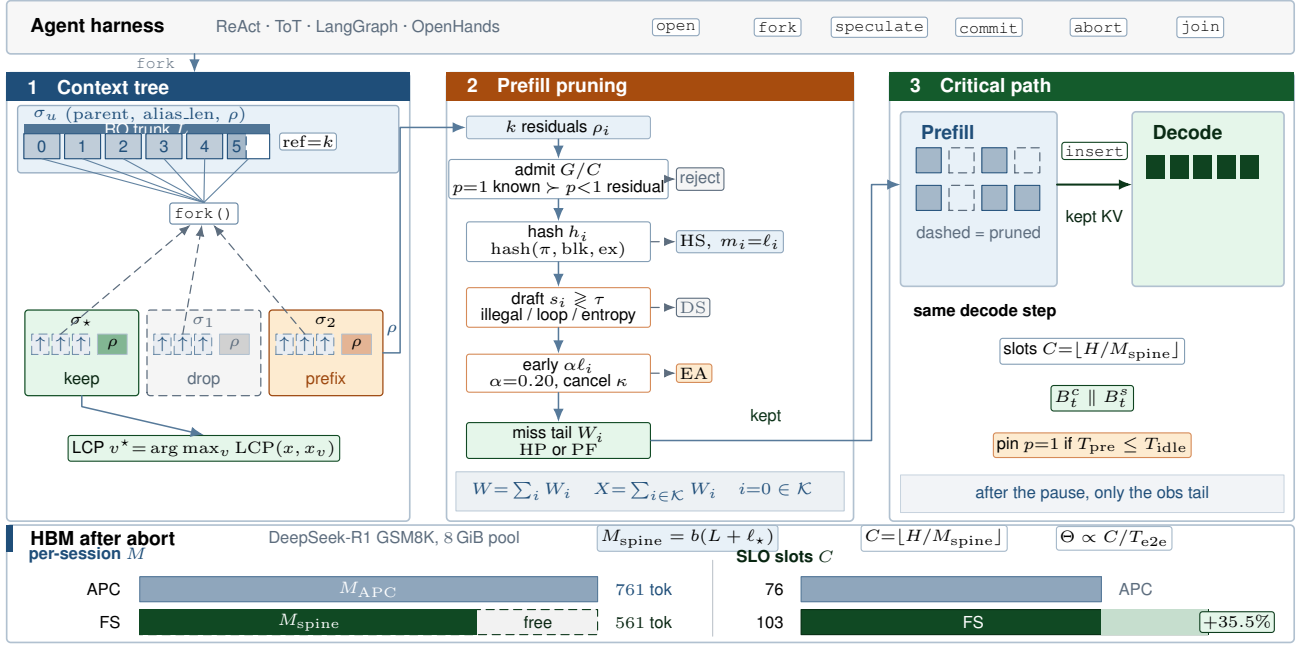
Figure 1. ForkServe architecture. (1) \sigma_u aliases one trunk; \text{fork} is O(1) ; (3) binds the winner. (2) One action a_i ((5)), fixed by the page-aligned match m_i . m_i = \ell_i issues no kernel; 0 < m_i < \ell_i prefills the miss; i \in \Lambda is withheld; every other miss is prefilled. X sums W_i over \mathcal{K} . (3) C = \lfloor H/M_{\text{spine}} \rfloor . After abort the live set is the spine, and the same pool admits 76 \rightarrow 103 sessions.
