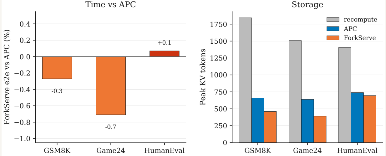
Figure 5: Setting B ( tp=2, n=4 ). Left: end-to-end time stays with APC ( -0.3\% , -0.7\% , +0.1\% ) because decode dominates T_{e2e} . Right: peak resident KV on the same runs. Branch-aware abort compresses storage to M_{spine} ( 0.70\times , 0.61\times , 0.94\times APC) at stable latency.
