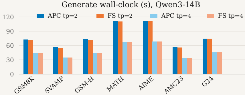
Figure 9: Qwen3-14B end-to-end generate time. Orange sits on blue in each tensor-width pair. Light bars (tp=4) are 0.61-0.64 \times the dark bars.
