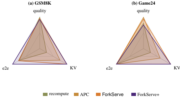
Figure 7. Four systems on Qwen3-8B ( n=80 , tp=2 , D=512 ). Spokes are normalized so the outer ring is the best value on that axis: quality, KV efficiency (inverse peak), and end-to-end speed. (a) GSM8K. (b) Game24. On the KV spoke, recompute lies inside the other three systems.
