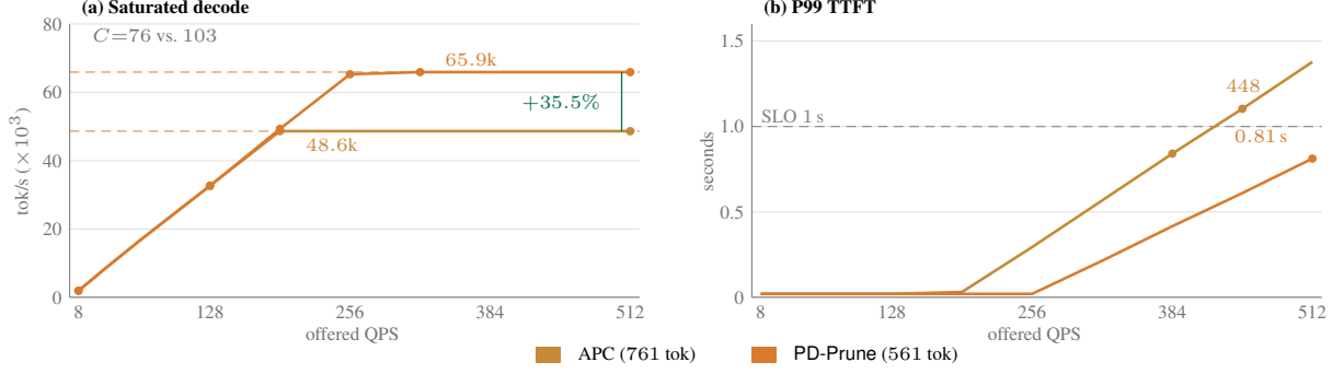
Figure 13: SLO sweep from the measured DeepSeek-R1 GSM8K peaks (761 APC tokens, 561 spine tokens, n=16 , k=4 ). An 8 GiB pool at 147456 bytes/token holds 76 and 103 trees. Each slot serves 640 tokens/s, so offered load saturates at 48640 and 65920 tokens/s. Under the same model the 1 s P99 TTFT line is crossed by APC at 448 QPS and is still met by PD-Prune at 512 QPS (0.81 s).
