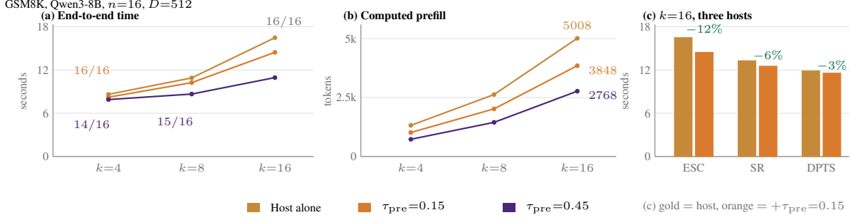
Figure 3: Prefill threshold on GSM8K (Tables 4, 6 and 14). (a) Wall-clock under ESC. Labels are any-finished. \tau_{\text{pre}}=0.45 is 14/16 at k=4 , 15/16 at k=8 , and 16/16 at k=16 . (b) Computed prefill, -23\% at 0.15 and -45\% at 0.45. (c) The same 0.15 threshold in front of each host at k=16 . Every row stays 16/16.
