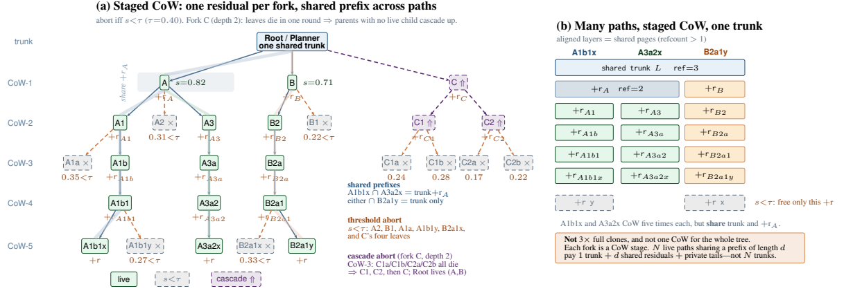
Figure 2: Context tree. (a) Each edge is one fork: the child aliases the parent and allocates only a residual ( +r ). Live paths share the trunk; A1b1x and A3a2x also share +r_A . All descendants of fork C are aborted at depth 2, so reclamation propagates up to C and stops at the root, which retains the live children A and B. (b) A shared layer is one physical page set with reference count greater than one; aborting a leaf frees only its residual.
