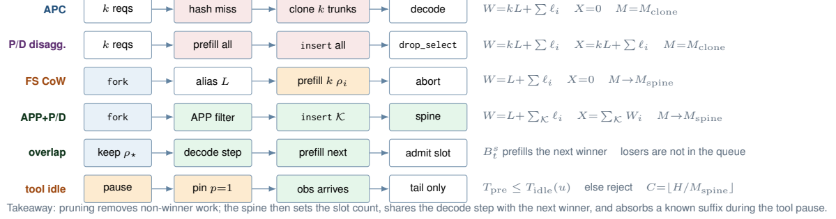
Figure 9: The admission rule and where it sits on the path. (a) a_i is the first match of (4). Only W_i for i \in \mathcal{K} reaches insert. (b) APC and baseline disaggregation copy the trunk. The alias removes L from W and from X . The overlap row prefills the next miss during decode. The tool-interval row prefills a suffix with p=1 while T_{\text{pre}} \leq T_{\text{idle}} .
