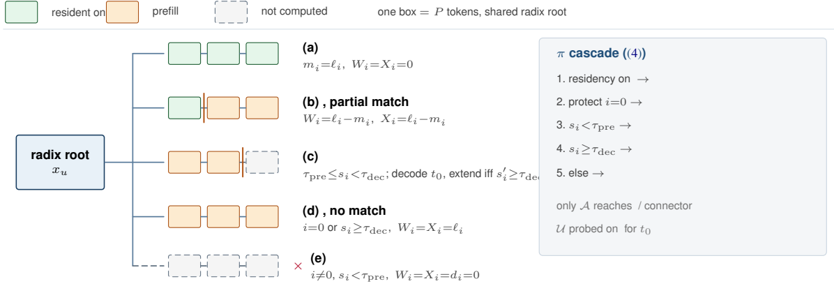
Figure 11: One radix tree, five actions ((4)–(6)). The root is the aliased trunk x_u . Each edge is one page of P tokens. Green pages are in H ; orange pages are prefilled; gray pages are withheld. (a) HS: m_i = \ell_i , W_i = X_i = 0 . (b) HP: 0 < m_i < \ell_i , W_i = \ell_i - m_i , X_i = \ell_i - m_i . (c) EA: m_i = 0 , F_i = 1 , W_i = \lceil \alpha \ell_i \rceil , X_i = 0 . (d) PF: m_i = 0 , i \notin \Lambda , \neg F_i , W_i = \ell_i . (e) DS: i \in \Lambda , W_i = X_i = 0 . A score below \tau with i \notin \Lambda is prefilled and probed (Algorithm 1).
