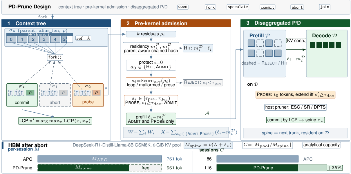
Figure 7: PD-Prune design. (1) CoW state: \sigma_u aliases one trunk, fork is O(1) in L , and LCP commit publishes x_* . (2) Controller policy \pi : observation o_i = (m_i^P, m_i^D, s_i) maps to a_i \in \{\text{HIT, ADMIT, PROBE, REJECT}\} ; only \mathcal{A} enters the GPU path. (3) Disaggregated execution: \mathcal{P} prefills the miss of \mathcal{A} , the connector ships decoder-missing pages, and \mathcal{D} runs the t_0 probe then the host pruner before LCP commit. Bottom: M_{\text{spine}} frees HBM and raises analytical session capacity.
