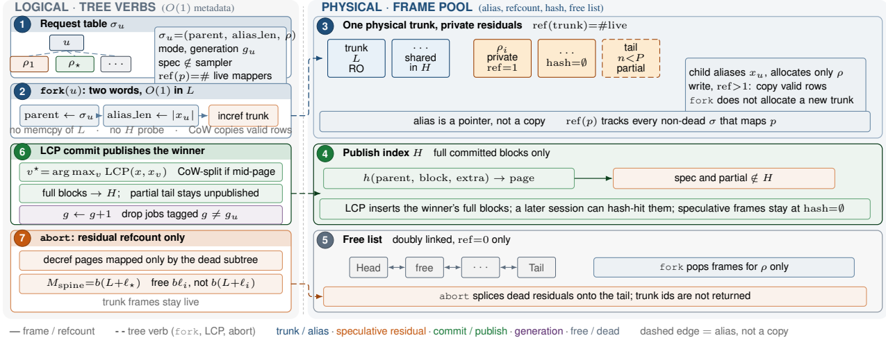
Figure 2. Context-tree page pool. A branch is an alias over the same three structures as a prefix-cache block pool: a request table, a hash index, and a frame free list. Left: \sigma_u stores (parent, alias_len, \rho ), a mode, and a generation ①. fork copies the two words and increments the trunk, O(1) in L , and does not probe H ②. LCP commit publishes full winner blocks and bumps g , so in-flight speculative jobs drop ⑥. abort decrefs residual pages only, leaving the spine M_{\text{spine}} = b(L + \ell_*) ⑦. Right: the trunk is one physical copy whose refcount is the number of live mappers; each child allocates only \rho , still at \text{hash} = \emptyset ③. H holds full committed blocks, so a later session can hash-hit the winner ④. The free list is doubly linked and stores only \text{ref} = 0 frames; fork pops residual frames and abort splices them back, never the trunk ⑤. A write with \text{ref} > 1 copies the valid rows of that page.
