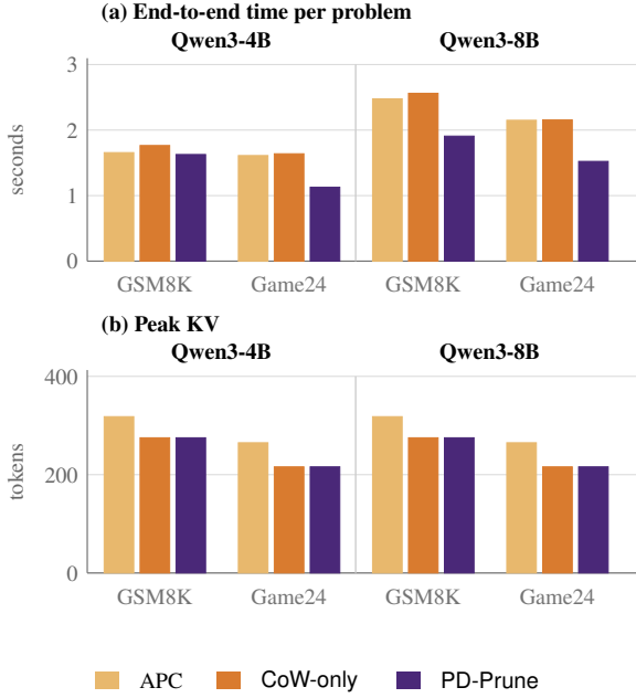
Figure 11: Three-step Tree-of-Thoughts ( n=16 , \text{tp}=2 ). (a) End-to-end seconds per problem; PD-Prune includes an answer-marker decode stop. (b) Peak KV of the live spine.
