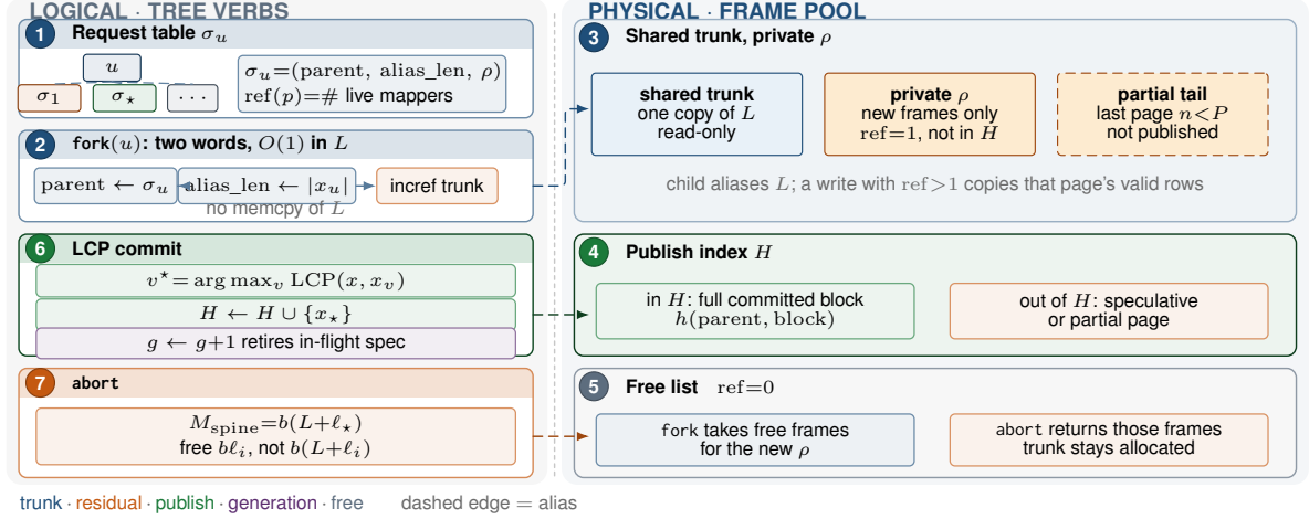
Figure 4: Context-tree page pool. fork aliases the trunk in O(1) and allocates only residual pages ①–③. Commit publishes x_* to the index ④⑥. abort returns residual pages only, so the live occupancy is M_{\text{spine}} = b(L + \ell_*) ⑤⑦.
