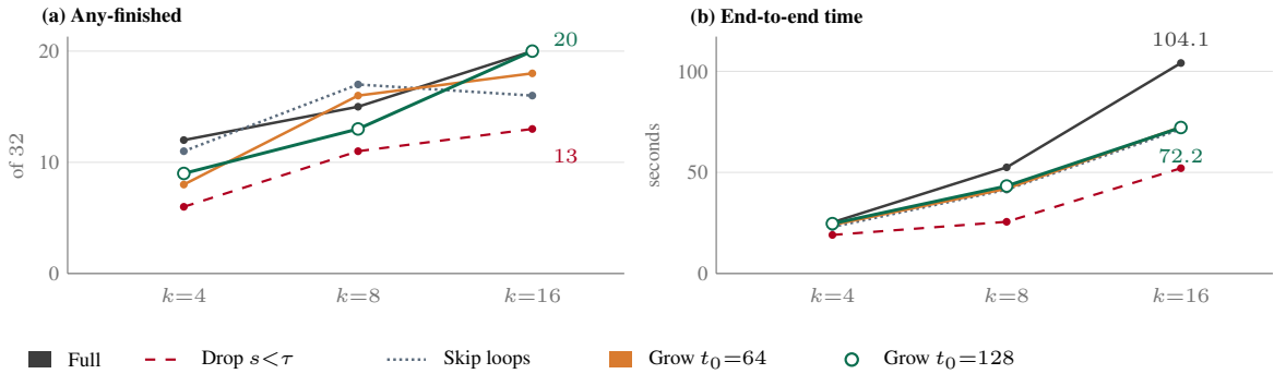
Figure 9: Probe admission on MATH-500 (Table 4). Blanket rejection is fast but loses coverage; a t_0=128 probe returns to 20/32 at k=16 in 72.2 s instead of 104.1 s.
