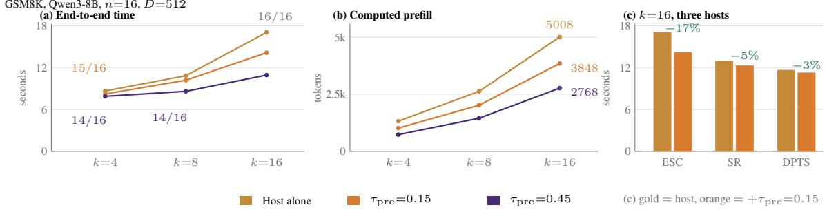
Figure 10: Admission threshold on GSM8K (Tables 2 and 3). (a) ESC wall-clock across k , labeled with any-finished coverage. (b) Computed prefill: -23\% at \tau_{\text{pre}}=0.15 and -45\% at 0.45 . (c) Reject-only admission in front of each host at k=16 .
