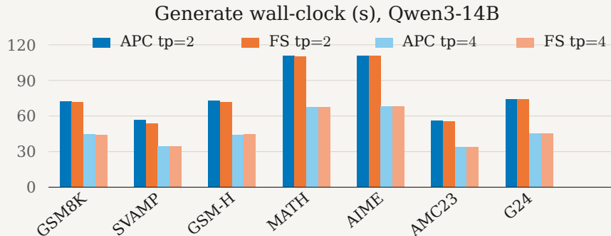
Figure 8: Qwen3-14B end-to-end generate time. Orange sits on blue in each tensor-width pair. Light bars (tp=4) are 0.61\text{--}0.64\times the dark bars.
