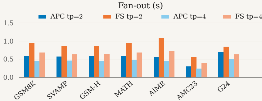
Figure 13: Fan-out (branch prefill plus abort). ForkServe is higher at matched W=L + k\bar{\ell} because of copy-on-write and abort. The gap is tenths of a second against 22–67s generate, so it does not move the accuracy or e2e comparison.
