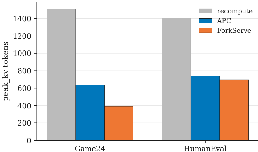
RL improve round 3, n = 4 , tp=4: peak KV (ok pairs)
