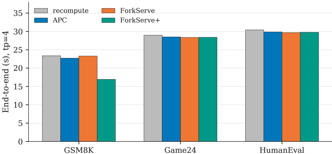
Setting M e2e: stop list only moves GSM8K
