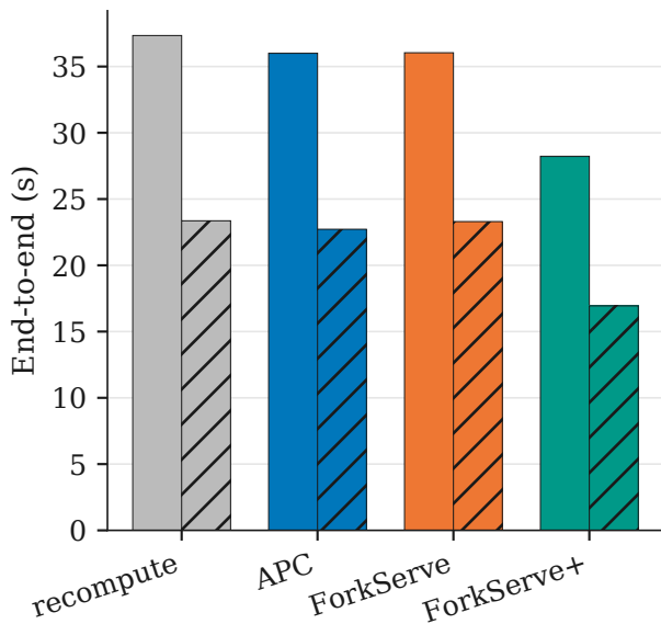
GSM8K wall-clock, n = 80
