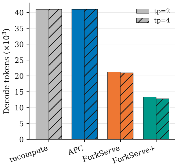
GSM8K emitted decode tokens
