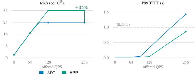
Figure 5. SLO sweep from measured DeepSeek GSM8K peaks. Left: saturated tok/s plateaus at C \times decode-rate (37 vs. 50 slots). Right: APC crosses the 1 s P99 line at 256 QPS; APP stays under it.
