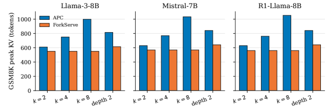
Figure 8. GSM8K peak KV versus branching ( n=16 , tp=2 , D=512 ). ForkServe+ matches the ForkServe bar. The spine is flat in k ; APC grows with the hashed union, so the ratio falls from 0.89–0.90 to 0.53–0.55.
