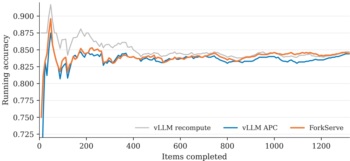
GSM8K official extractor, running score
