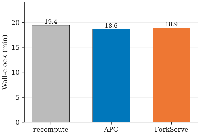
GSM8K generate time (first to last chunk)
