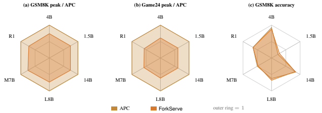
Figure 7. APC versus ForkServe on six models ( n=40 , tp=2 ). Each spoke is one family. (a) (b) Peak KV divided by the APC peak, so the outer ring is APC and the inner polygon is ForkServe. (c) GSM8K accuracy on the same scale. ForkServe+ shares the spine in (a) and (b).
