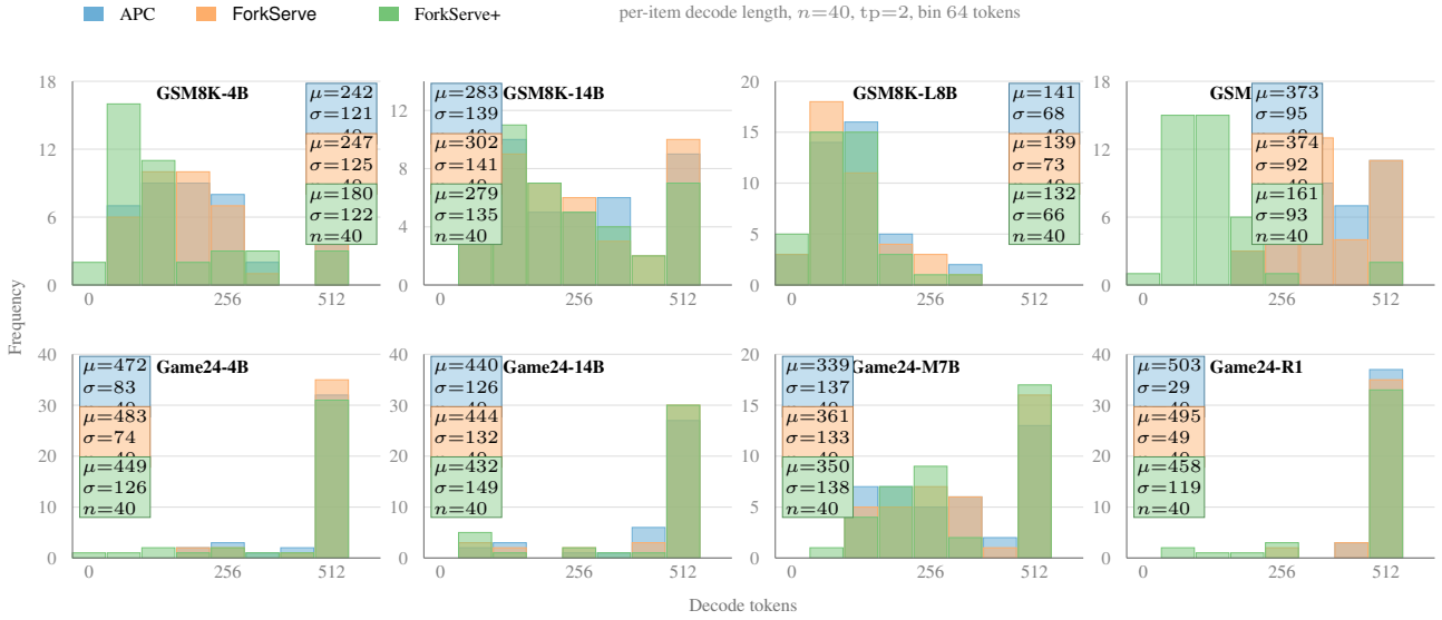
Figure 8. Per-item decode-length histograms ( n=40 , tp=2 , D=512 ). Each panel overlays APC, ForkServe, and ForkServe+ (bin width 64). Boxes report \mu , \sigma , and n . GSM8K (top): ForkServe+ left-shifts Qwen3-4B; Llama-3-8B stays near APC. Game24 (bottom): mass sits at the budget—the marker list does not transfer. Llama-3-8B Game24 is omitted (all lengths 1); Mistral-7B is shown instead.
