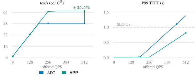
Figure 5. SLO sweep from measured DeepSeek GSM8K peaks. Left: saturated tok/s plateaus at C \times decode-rate (76 vs. 103 slots). Right: APC crosses the 1 s P99 line at 448 QPS; APP stays under it through 512.
