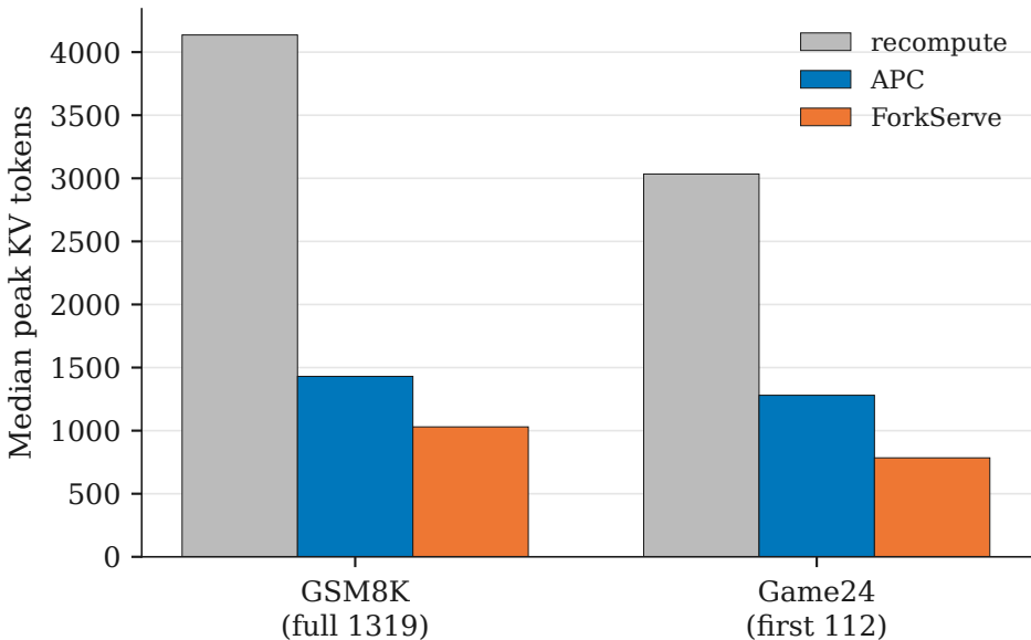
Committed-spine KV vs prefix cache vs recompute
