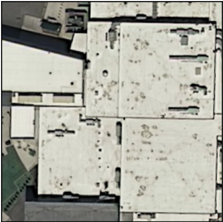
image buildings93
