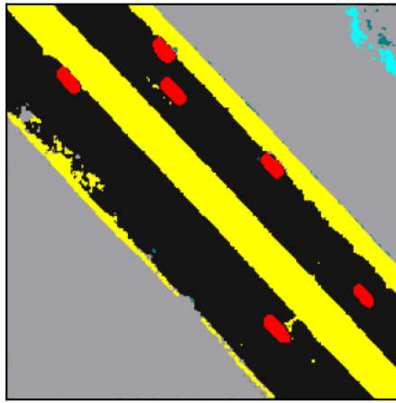
baseline \tau=0.1 71.8
