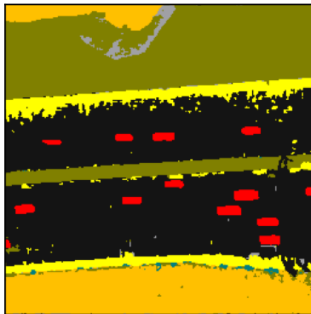
baseline \tau=0.1 18.8
