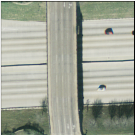
image freeway58
