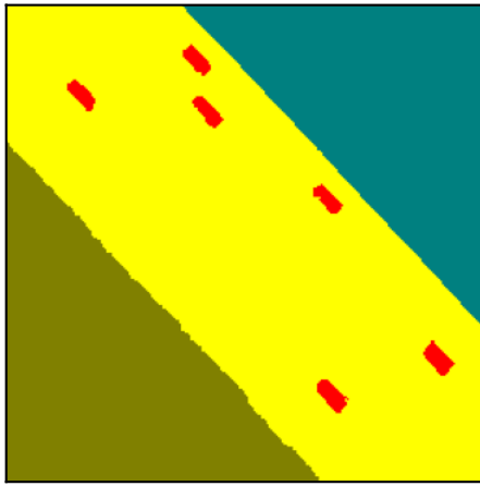
ground truth
