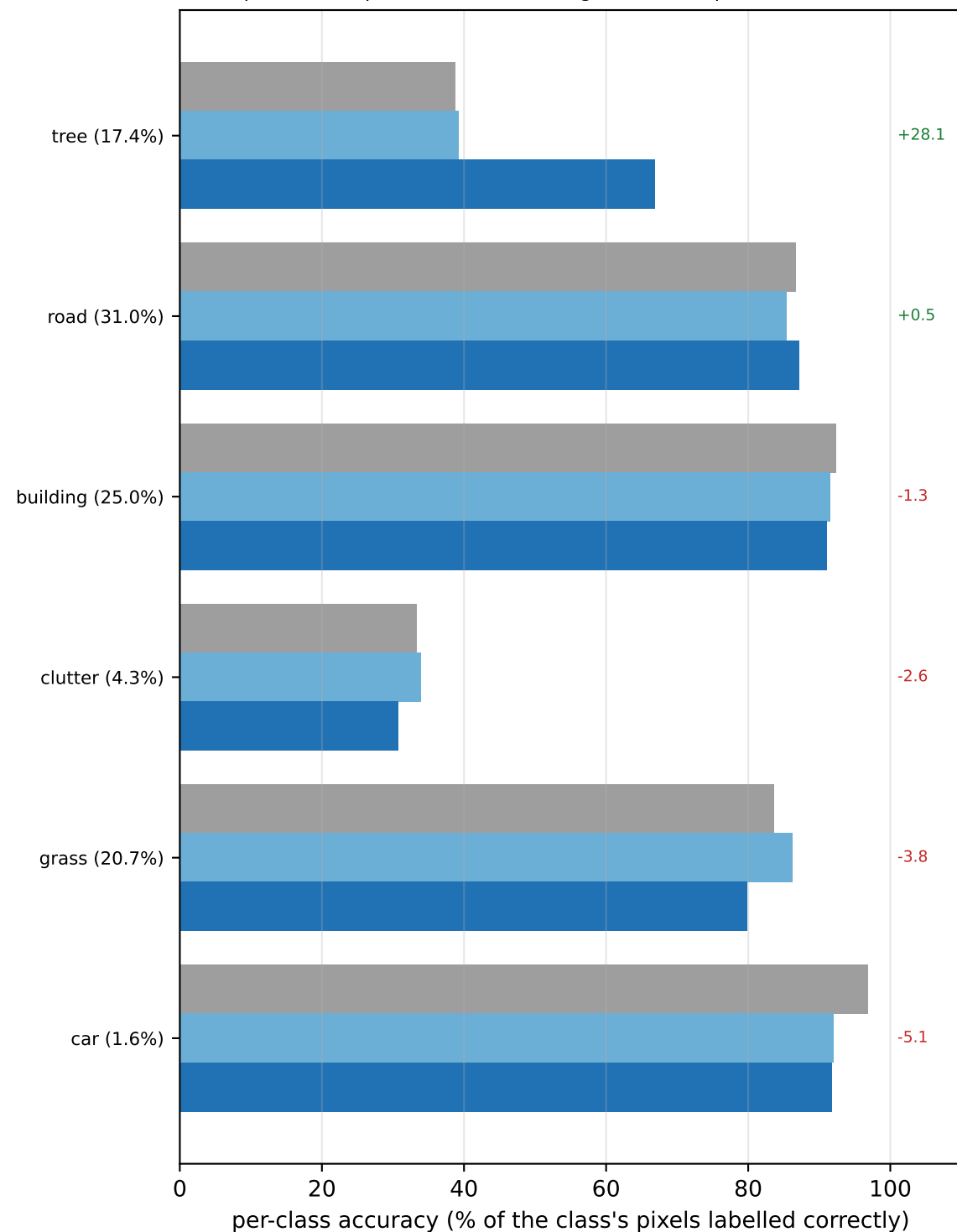
potsdam — per class (C – A at right; share of pixels in brackets)
