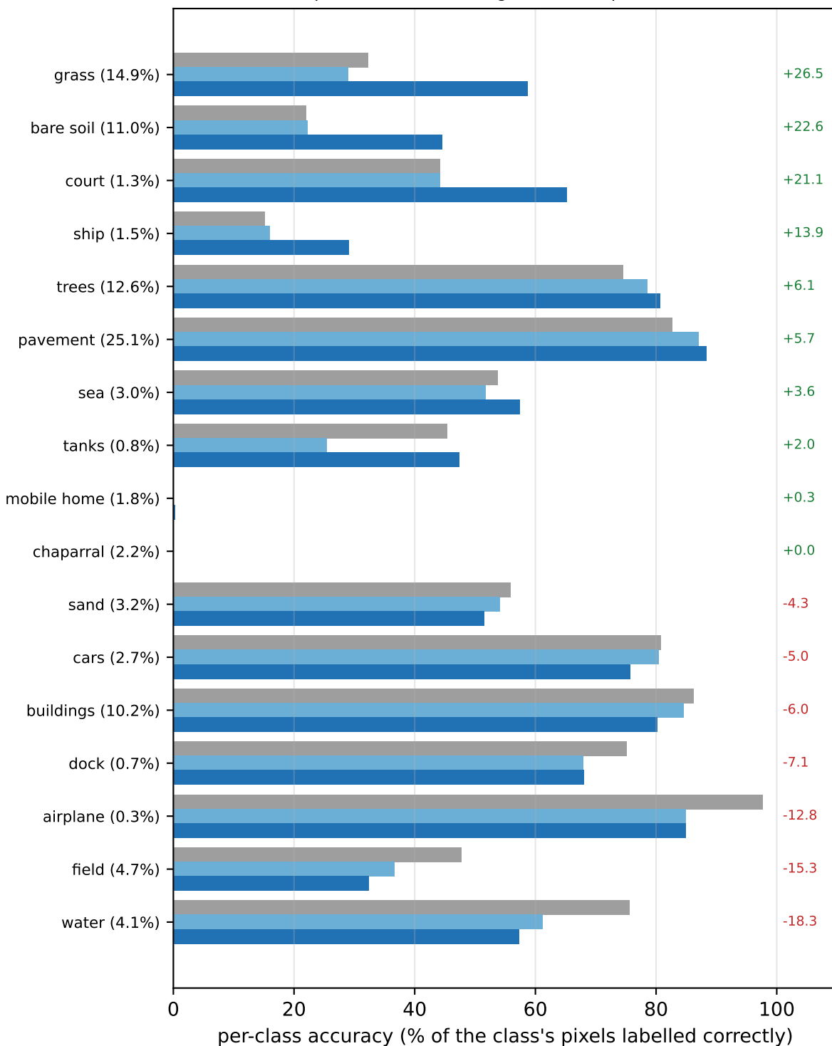
dlrds — per class (C – A at right; share of pixels in brackets)
